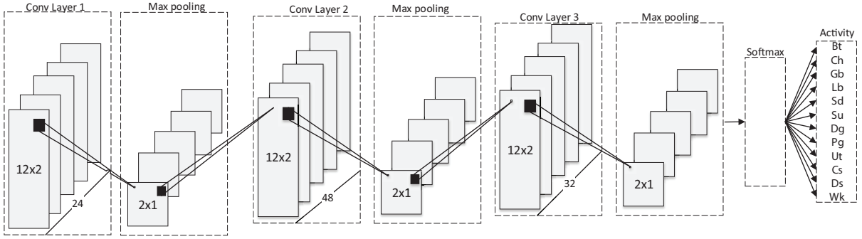
Fig. 1 Proposed convolutional neural network. All convolutional filters capture the temporal (by height) and the pattern among the accelerometer axes (by width).
